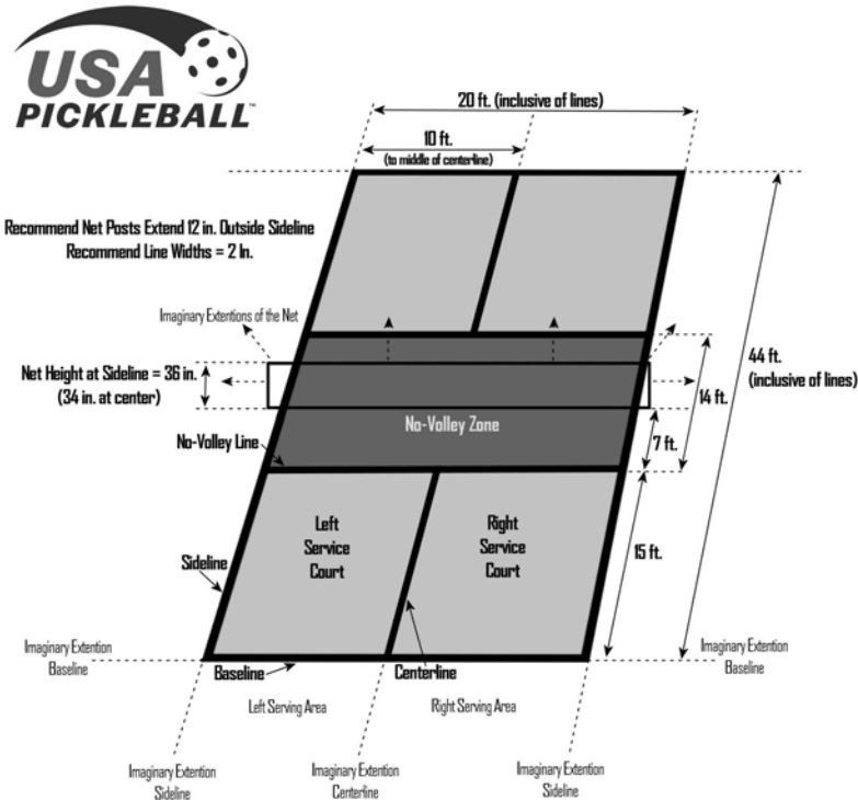
Figure 3-1: Court Specifications
